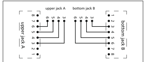
Schaltbild 906807 Connection Diagram 906807
